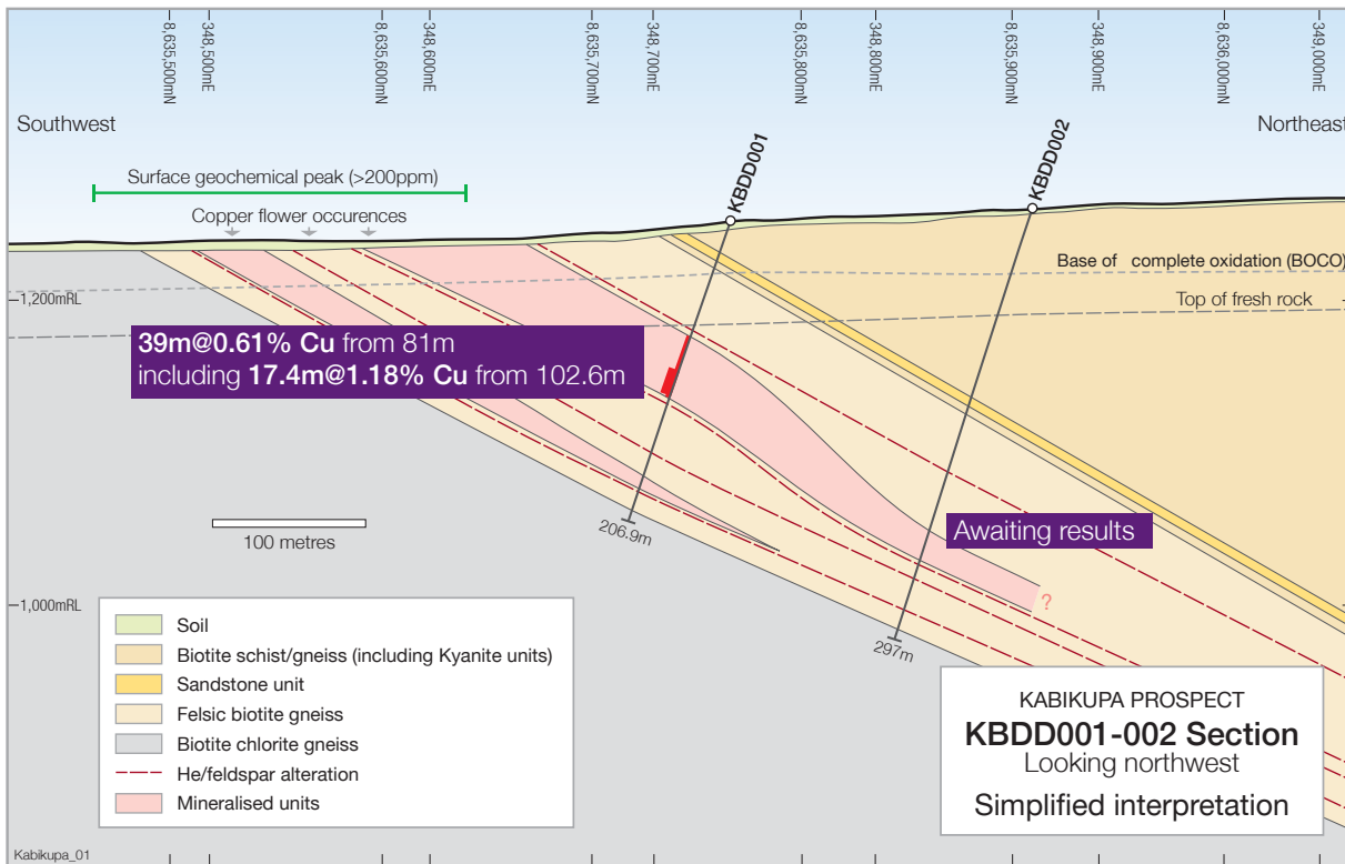
Figure 3 Preliminary interpretive cross section through the Kapikuba prospect.
